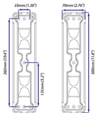
Wall Plate Dimensions
